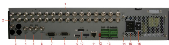
Rear Panel of DS-8116HFI-ST
