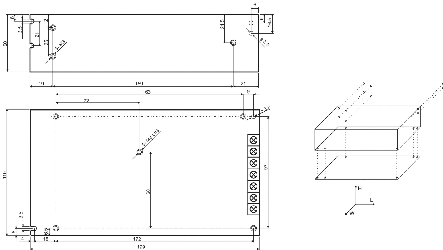
Fig.2. Dimensions of power supply.
