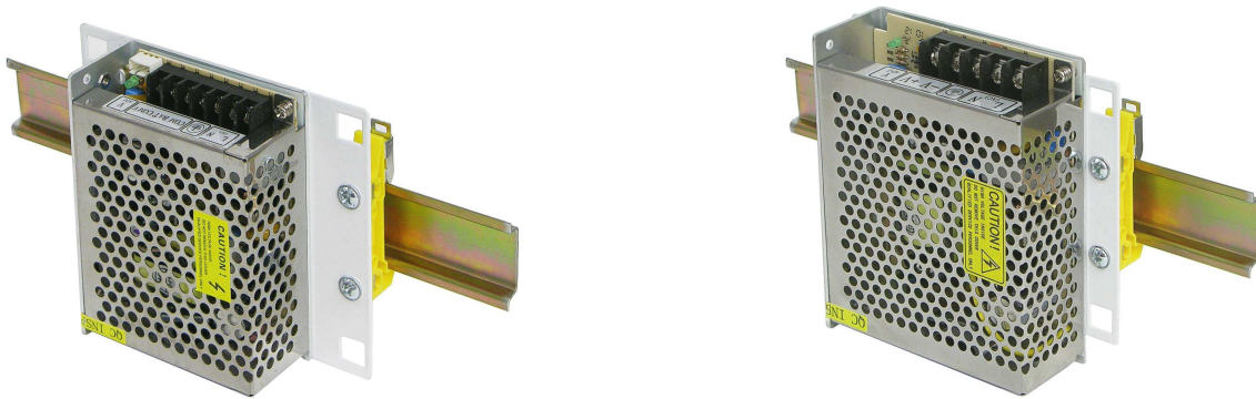
Fig. 2. Example of power supply mounting: PSB201202 and PS401203.
